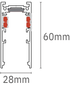
SURFACE TRACK Track System
