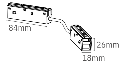
CORNER CONNECTOR
