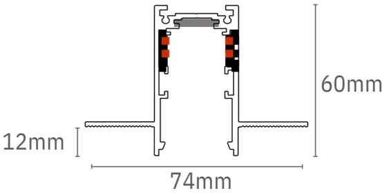
RECESSED DEEP TRACK
